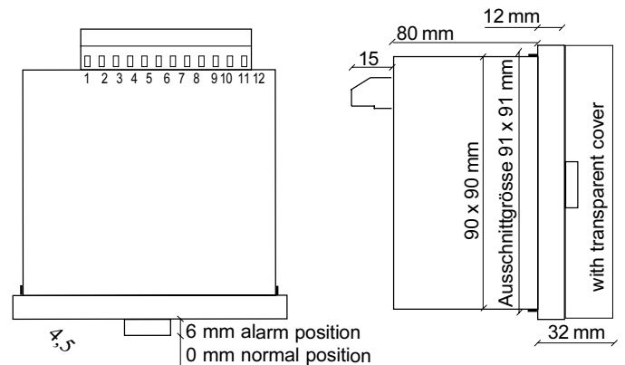
Dimensions of external limiting resistor Execution 'Standard'
