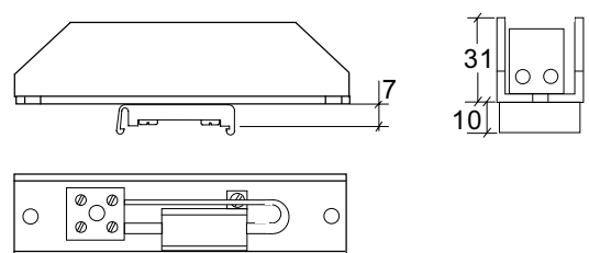
Dimensions of external limiting resistor Very special execution for mounting on DIN rail
