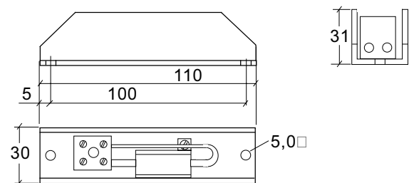
Dimensions of external limiting resistor Execution 'Standard'
